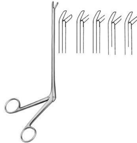
Cushing MDC-8-139-01 Laminectomy Rongeur jaw 2 x 10 to 4 x 10 mm straight shaft length 180 mm
